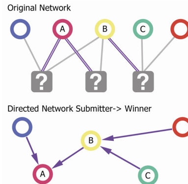
Figure 3: Users are denoted by colored circles and tasks are denoted as question marks. Purple double lines are "wins"; grey lines are "non-winning" submissions. The user prestige network is derived as follows: if users A and B participate in the same task and A wins, then we add an edge from B to A.
