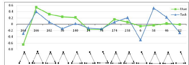
Figure 7: Motif profiles of users and tasks in the Design category. The Y-axis is the normalized z-score of the frequency deviation from the random network.
